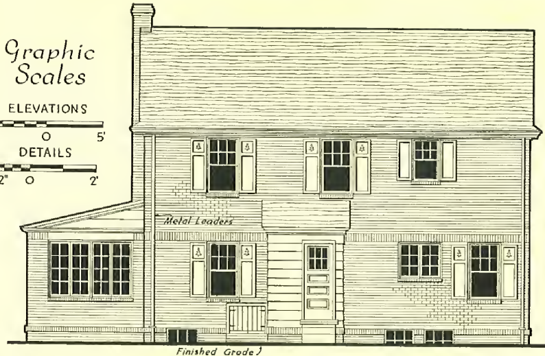
Rear Elevation
